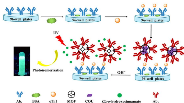
Fig. 4 Schematic diagram of cTnI detection by fluorescence immunosensor with signal amplification. Reproduced from ref. 38 with permission from American Chemical Society.
