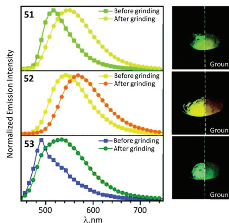
Fig. 11 Solid-state emission spectra of 51–53 before and after grinding using \lambda_{\text{exc}} 425 nm; photographs taken under UV lamp illumination ( \lambda_{\text{exc}} 365 nm). Adapted with permission from ref. 49. Copyright (2020) The Royal Society of Chemistry.
