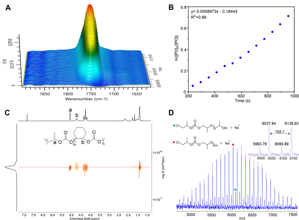
Fig. 2 (A) In situ FTIR surface image monitoring the formation of polycarbonate (1750 cm -1 ). (B) The plot of ln([PO] 0 /[PO]) versus time under the polymerization conditions: PO : 5 = 100 : 1, CO 2 10 Bar, and 60 °C. (C) DOSY NMR of the PPC- b -PCHC block copolymer. (D) MALDI-TOF MS of the polycarbonate obtained in the presence of catalyst 5.
