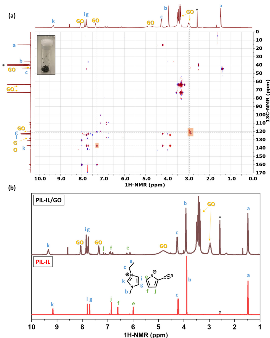
Fig. 6 (a) HMBC spectra showing the molecular interactions between PIL, IL, and GO components. Inset shows the images of PIL-IL/GO material collected by scraping off the top selective layer from the PIL-IL/GO on b PES/PET to redisperse in DMSO- d_6 for HMBC NMR. (b) ^1\text{H} -NMR of the PIL-IL/GO and PIL-IL gel. The GO peaks, from high field to down field, are likely due to the native alkyl-CH ( \sim 3 ppm), OH (4.7 ppm), aromatic-CH ( \sim 7 ppm) functionalities that are captured due to their interaction with the IL. The NMR of pure GO is shown in Fig. S8.†
