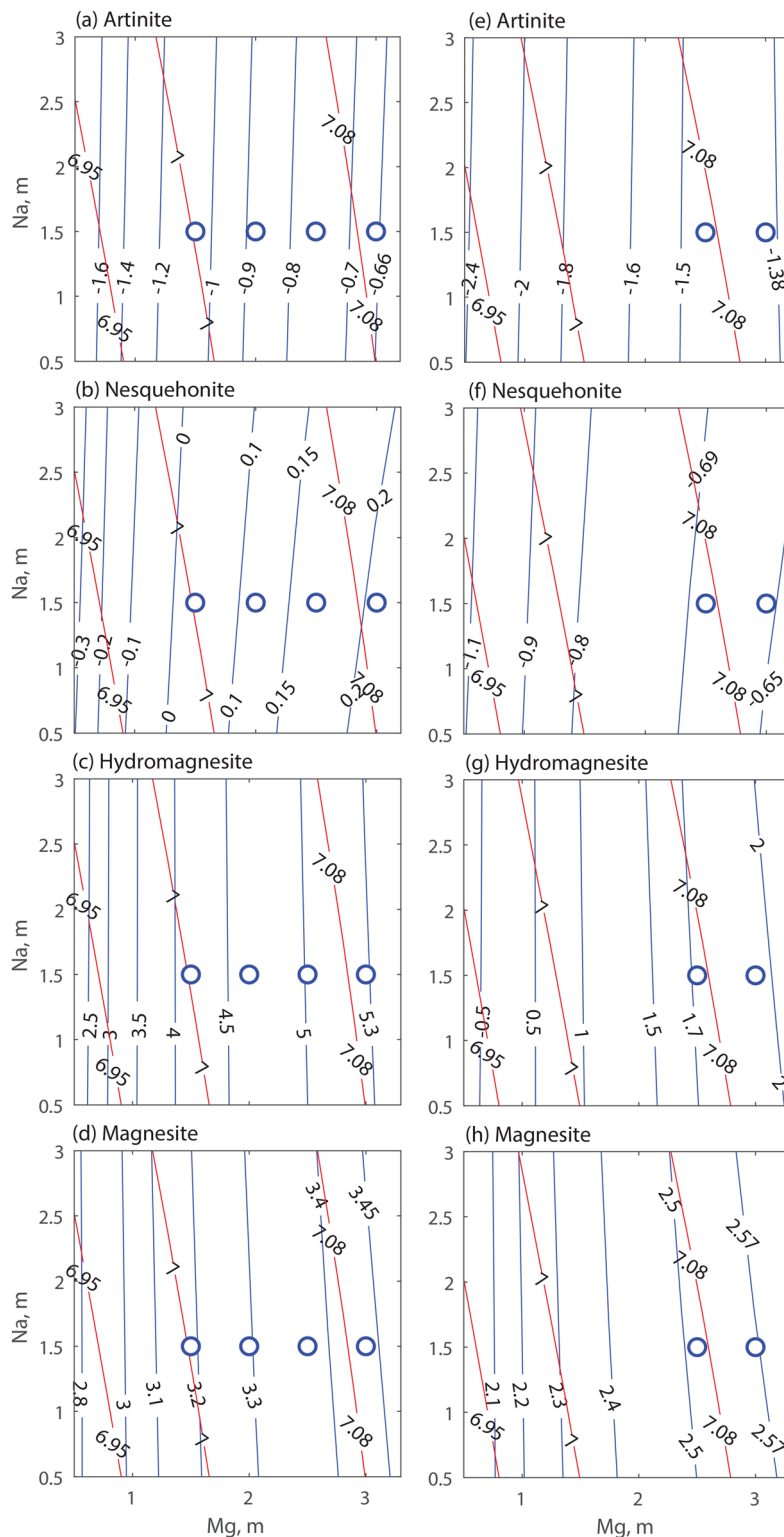
Fig. 3 Contours of pH (red) and SI (blue) calculated at 25 °C at p CO 2 equal to (a–d) 1 and (e–h) 0.1 bar. The dots indicate the applied experimental conditions.
