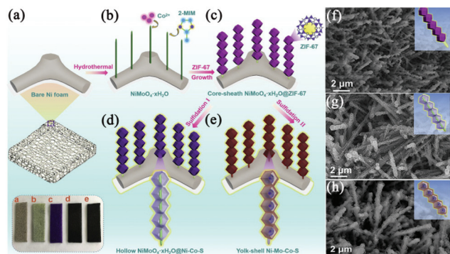
Fig. 8 (a–e) Schematic illustrations of the synthesis of yolk-shell Ni-Mo-Co-S NCAs on NF. SEM images of (f) \text{NiMoO}_4 \cdot x\text{H}_2\text{O} @ \text{ZIF-67} , (g) hollow \text{NiMoO}_4 \cdot x\text{H}_2\text{O} @ \text{Ni-Co-S} NCAs and (h) yolk-shell Ni-Mo-Co-S NCAs. Reprinted with permission from ref. 98, Copyright 2020, Elsevier.
