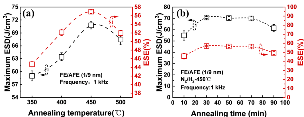
Fig. 3 The maximum ESD and corresponding ESE of the capacitor with the FE (1 nm)/AFE (9 nm) stack: (a) at different annealing temperatures for 30 \text{ min} ; (b) at 450 \text{ }^\circ\text{C} for different annealing times. Ten devices are measured for each sample.
