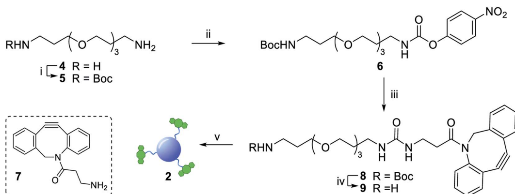
Scheme 1 Reagents and conditions: (i) Boc 2 O, DCM, 4 h, 0 °C to rt, 99%; (ii) 4-nitrophenyl chloroformate, Py, DCM, 3 h, 0 °C to rt, 87%; (iii) 7, Py, DIPEA, DMF, 63%; (iv) TFA, DCM, 1.5 h, rt, 86%; (v) 3, HATU, DIPEA, DMF, 5 h, rt.
