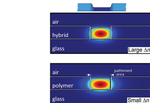
Fig. 4 Finite-element modelling (see ESI ^\dagger for details) illustrating the improvement of energy localization in the intensity of the TE fundamental mode for a wavelength of 550 nm in a co-planar channel waveguide if a resolution of 1 \mu m were to be achieved via local annealing of the PVAL/titanium oxide hydrate hybrid (top panel). This is compared to currently used systems as described in, e.g., ref. 9–13 (bottom panel), assuming an air top cladding ( n = 1 ) and a glass bottom cladding ( n = 1.5185 ) in both scenarios. The central section was modelled with an index difference of +0.10 relative to the neighbouring areas ( n = 1.73 for the core; n = 1.63 for the untreated regions), as achievable by heat treating the hybrid material, while \Delta n = 0.05 was used to model currently available optical polymers (core: n = 1.68 , side cladding n = 1.63 9–13 ). Dimensions used were based on a high-refractive index core of 1 micron width and 575 nm in height (in case of the hybrid to take the shrinkage upon heat exposure into account; the height used for the untreated areas was 660 nm, vs. a 660 nm height for the whole structure for the reference polymer material).
