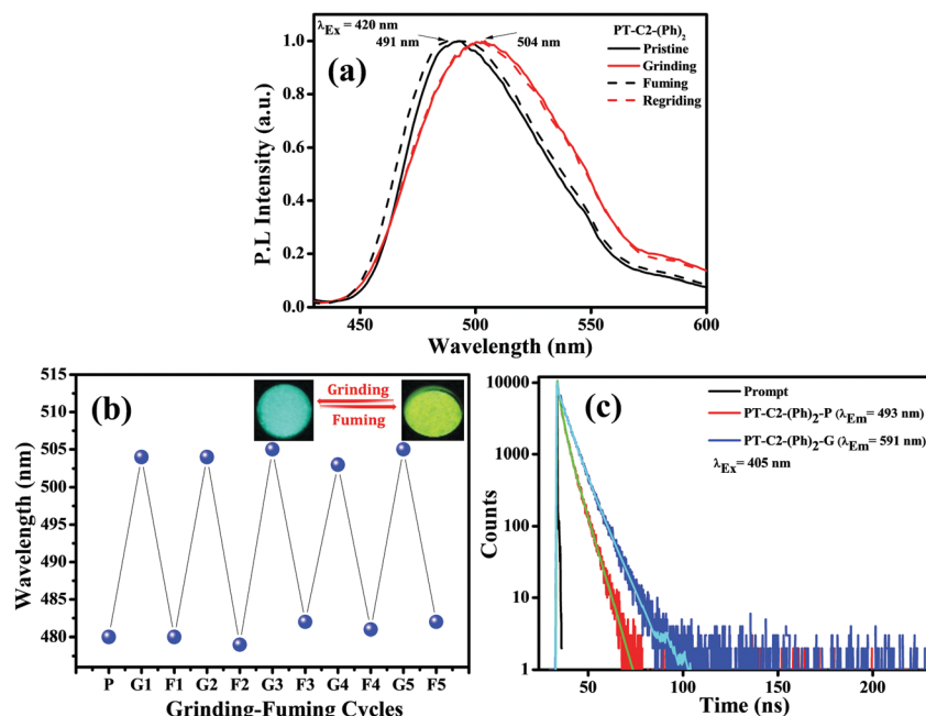
Fig. 6 (a) Fluorescence spectra ( \lambda_{\text{Ex}} = 420 nm) of PT-C2-(Ph) 2 upon grinding–fuming cycles, (b) emission color alteration of PT-C2-(Ph) 2 upon grinding–fuming cycles and (c) time-resolved fluorescence decay of PT-C2-(Ph) 2 in its pristine and ground state ( \lambda_{\text{Ex}} = 405 nm).
