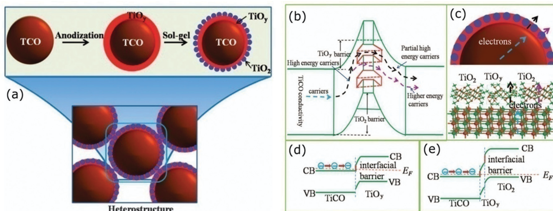
Fig. 7 (a) Schematic illustration of the formation of the \text{TiC}_{1-x}\text{O}_x@(\text{TiO}_y-\text{TiO}_2) heterostructures via anodization process. The mechanism of carrier transport through the double-barrier: (b) carrier paths where the first interfacial \text{TiO}_y barrier selectively scatters low-energy carriers and the \text{TiO}_2 barrier further scatters partial high-energy carriers, (c) transport schemes of the carriers in the heterostructures and at the interface, (d) and (e) show the band diagrams of the all-oxide \text{TiC}_{1-x}\text{O}_x@(\text{TiO}_y-\text{TiO}_2) heterostructured interfaces. Reproduced with permission from ref. 110, Copyright 2015 Nature Publishing Group.
