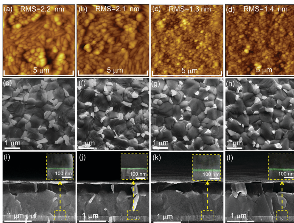
Fig. 3 AFM images of the surface morphology of (a) c-SnO 2 , (b) c(Li)-SnO 2 , (c) c-NP-SnO 2 and (d) c(Li)-NP-SnO 2 ETLs. Top and cross-sectional SEM images of perovskite thin films deposited on (e and i) c-SnO 2 , (f and j) c(Li)-SnO 2 , (g and k) c-NP-SnO 2 and (h and l) c(Li)-NP-SnO 2 ETLs.
