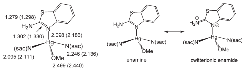
Chart 3 A summary of important bond lengths in [\text{Hg}(\text{sac})_2(\text{abt})\text{L}] ( 2a–b ) ( \text{L} = \text{MeOH}, \text{DMSO} ) and resonance hybrids for \text{Hg}(\text{II}) -abt complexes.
