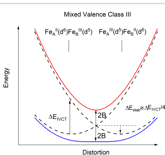
Fig. 11 Configuration energy diagram (schematic) for 3' in the limit of a complete delocalization of the extra electron over the two iron sites ( \text{Fe}^{2.5+}_\mu\text{Te}_2\text{Fe}^{2.5+} , Class III).
