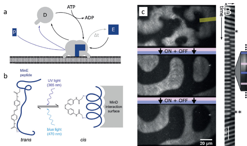
Fig. 6 Entrainment of Min-protein patterns based on a photoswitchable MinE peptide. (a) Monomeric MinD in solution forms a dimer that attaches to the membrane upon binding ATP. (b) Upon illumination with UV, the MinE peptide associates with membrane-bound MinD, causing hydrolysis of ATP followed by release of MinD from the membrane. (c) Periodic illumination of the sample synchronizes the patterns with the light pulses. Reproduced from ref. 89 with permission from the Wiley-VCH publishing group, Copyright 2018.
