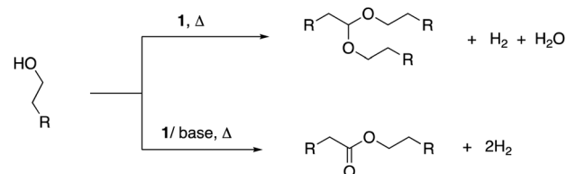
b) Reaction pathway for acetal formation
