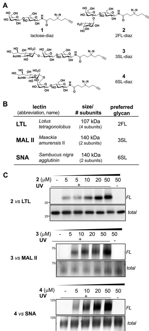
Fig. 1 HMO probes bind to purified plant lectins. (A) Chemical structures of HMO probes 1–4 . (B) Plant lectins, such as LTL, MALII, and SNA are oligomeric proteins known to exhibit preferences in glycan binding. (C) Analysis of probe engagement with plant lectins. Photo-crosslinking was found to be UV- and dose-dependent.
