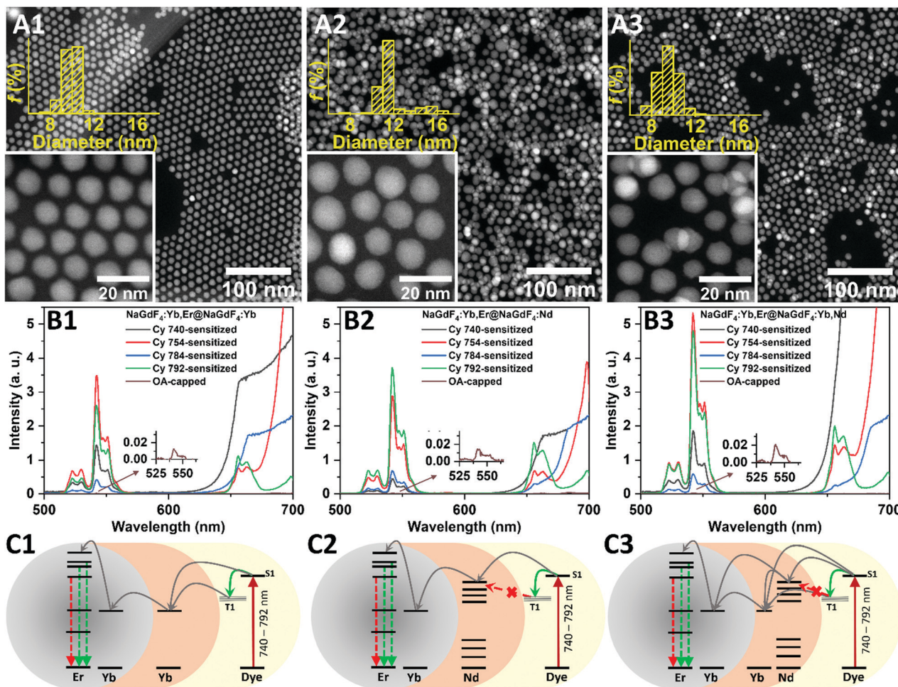
Fig. 5 (A1–A3) High-angle annular dark-field scanning transmission electron microscopy (HAADF-STEM) micrographs and size-distribution histograms, (B1–B3) UC luminescence spectra in \text{CD}_3\text{OD} , and (C1–C3), schematic of energy-transfer pathways of different types of dye-sensitized core@shell UCNCs (1, \text{NaGdF}_4:\text{Yb},\text{Er}@/\text{NaGdF}_4:10\%\text{Yb} ; 2, \text{NaGdF}_4:\text{Yb},\text{Er}@/\text{NaGdF}_4:30\%\text{Nd} ; and 3, \text{NaGdF}_4:\text{Yb},\text{Er}@/\text{NaGdF}_4:10\%\text{Yb},30\%\text{Nd} ). The dye-sensitization processes were performed under Ar, without further purification processes. Cy 740-, Cy 754-, Cy 784-, and Cy 792-sensitized, and OA-capped UCNCs were excited with 740, 754, 784, 792, and 980 nm lasers, respectively (excitation power of 75\text{ W cm}^{-2} ).
