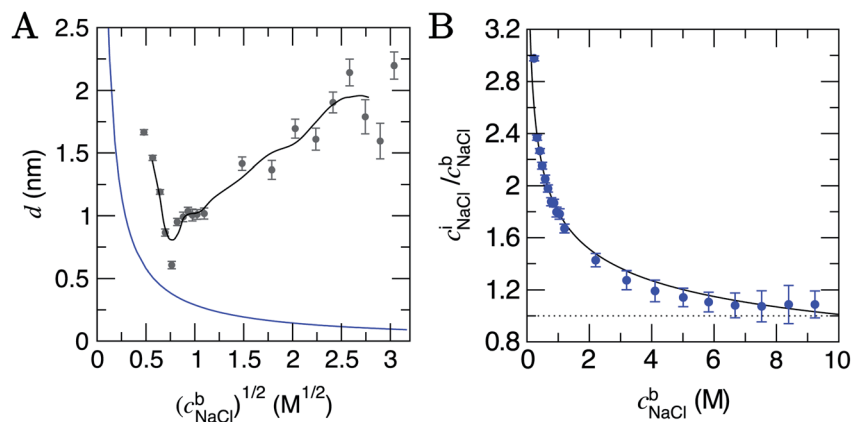
Fig. 2 (A) The depth of the double layer region, d , in \text{C}_{\mu}\text{MD} simulations with varying scaled bulk ion concentrations, (c^b) . The grey points provide the size of the double layer in x , with error bars indicating uncertainties of one standard deviation in the data. The black line provides a moving average for the data. Note that the minimum value of x for the solution phase (with reference to Fig. 1) was taken to be the mid-point between the carbon surface and the minimum value in ion concentration profiles: x \approx 1.35 nm. Also shown in the figure is the blue curve which is the Debye length (see ESI Section B†). (B) Provides the normalised, mean interface ion concentrations ( c_{\text{NaCl}}^i ) in a 1.5 nm solution region close to the graphite surface vs. the bulk concentration of ions. The black line is a fit to the data with functional form 1.8(c_{\text{NaCl}}^b)^{-0.25} and error bars show uncertainties of one standard deviation.
