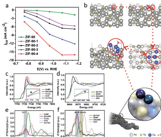
Fig. 7 (a) j_{CO} values of ZIF-90, ZIF-90-1, ZIF-90-2, ZIF-90-3, and ZIF-90-4. Reproduced from ref. 86 with permission from the Royal Society of Chemistry, copyright 2020. (b) A schematic illustration of Cu-doped Pd_{10}Te_3 nanowires. Reproduced from ref. 91 with permission from Springer Nature, copyright 2019. (c) K-edge XANES and (e) Fourier-transform EXAFS spectra of ZnCoNC. (d) K-edge XANES and (f) Fourier-transform EXAFS spectra of ZnCoNC. Reproduced from ref. 27 with permission from John Wiley and Sons, copyright 2020.
