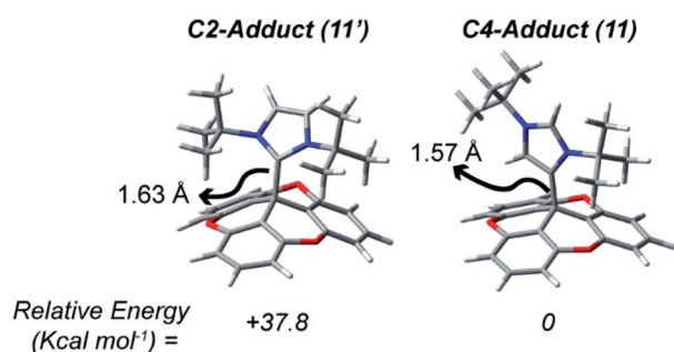
Fig. 6 Relative energy and bond \text{TOTA} – \text{NHC} bond distances from the calculated DFT models of 11 and 11' .
