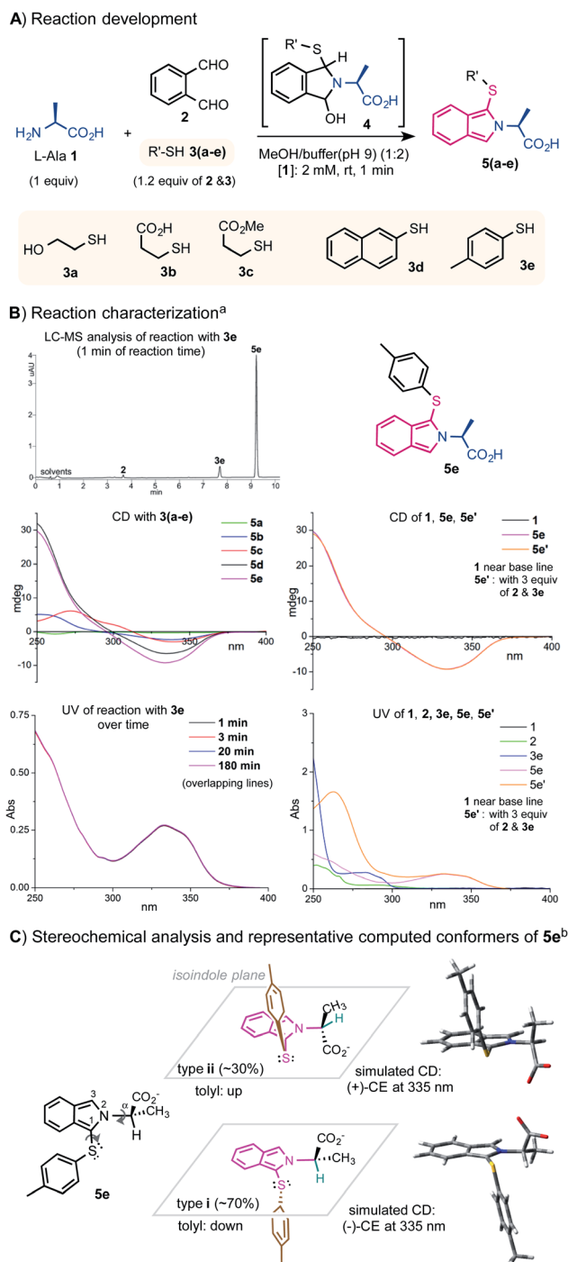
Fig. 1 Labeling of L-Ala with oPA and thiols for chiroptical sensing by CD/UV. (A) Reaction development. (B) Reaction characterization; a) reaction mixture was diluted 7 times and samples were measured at 0.285 mM for CD and UV. (C) Stereochemical analysis and representative computed conformers of 5e ; b) DFT calculations were performed at the M062X/6-311+G(d,p) level, see the ESI† for details.
