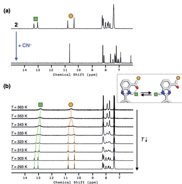
Fig. 5 (a) ^1\text{H} NMR spectra of 2 (4.0 mM) prior to (top) and after (bottom) the addition of NaCN (10 equiv.) in DMSO- d_6 ; T = 298 K. (b) Variable-temperature (VT) ^1\text{H} NMR spectra of 2 (4.0 mM) in DMSO- d_6 measured at T = 293 – 363 K.
