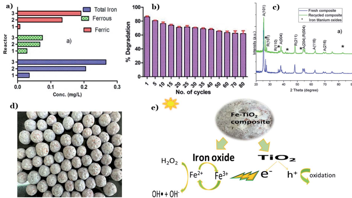
Fig. 17 Contents of total iron, ferrous, and ferric ions leached out from the beads with the passage of every reactor throughout the photo-degradation of MTZ (a); catalytic stability of composite beads for MTZ degradation (b); XRD patterns of fresh and recycled composite (c). This figure has been reproduced (adapted) from ref. 122 with permission from Elsevier, copyright 2019. Actual photograph of Fe–TiO 2 immobilized composite (FS and FA) beads (d); diagram illustrations of possible synergistic effect in dual-process under solar irradiation (e). This figure has been reproduced (adapted) from ref. 121 with permission from Elsevier, copyright 2017.
