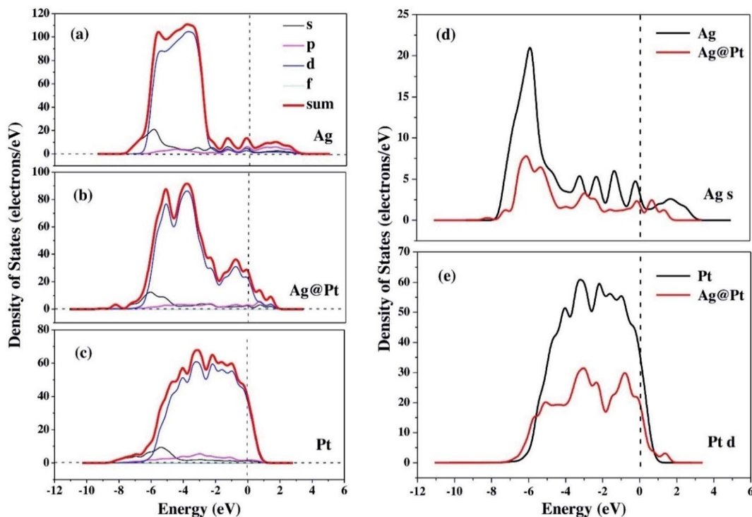
Fig. 20 The TDOS and partial density of states (PDOS) of Ag (a), Ag@Pt (b) and Pt (c) nanoparticles, the s-electron PDOS of Ag cores (d) and the d-electron PDOS of Pt shells (e), respectively. This figure is reproduced from ref. 138 with permission from Elsevier, copyright 2017.
