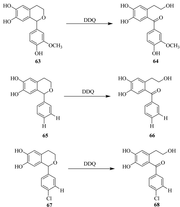
Scheme 29 Deprotection of hydroxyisochromans by DDQ.
