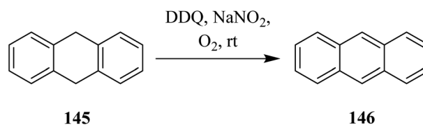
Scheme 52 Dehydrogenation of dihydroarenes by DDQ.
