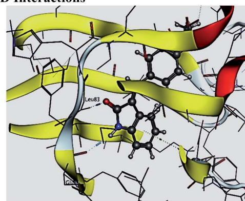
Fig. 8 2D and 3D ligand interactions of (A) co-crystallized sunitinib (Z) with CDK2, (B) 5a (Z-diastereomer), (C) compound 6c (E-diastereomer). All ligands are docked into the active site of CDK2 (PDB ID: 3T11).
