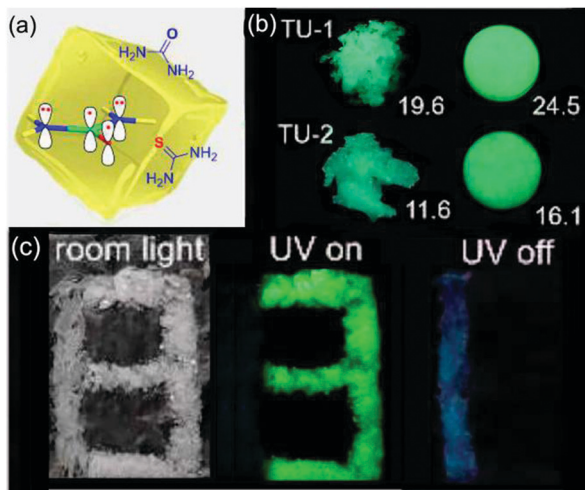
Fig. 25 (a) Structures of urea and TU and their delocalized \pi_6 system. (b) Photographs of TU-1, TU-2, and their tablets taken under 312 nm UV light. \phi values (%) of the samples are also given. (c) Pattern "8" comprising urea (blue part) and TU-1 (green part) crystals taken under room light, 312 nm UV light, and after ceasing the UV irradiation. Reprinted with permission from ref. 40. Copyright 2020, John Wiley and Sons.
