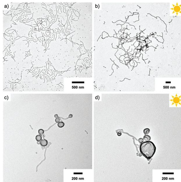
Fig. 6 Morphologies of PEO 113 -ONB- b -PS x BCPs in water. TEM of P2 cylinder micelles at c = 0.1 \text{ mg mL}^{-1} before irradiation (a) and after irradiation (b). TEM of P3 vesicles at c = 0.1 \text{ mg mL}^{-1} before irradiation (c) and after irradiation (d).
