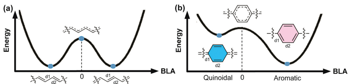
Fig. 1 Energy diagrams of the ground states of the infinite chain of (a) polyacetylene and (b) poly- para -phenylene (PPP) as a function of BLA, which is defined as (d_2 - d_1)/2 . Reproduced (adapted) from ref. 8 with permission from John Wiley and Sons.
