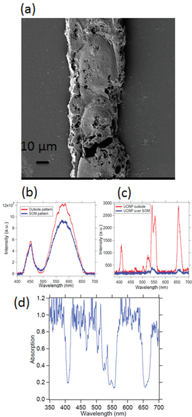
Fig. 9 The (a) deposited SOM pattern and (b) the corresponding absorption spectra taken with a broadband lamp and (c) taken with a UCNP source. The (d) shows the absorption ratio due to SOM pattern taken with UCNP. Typically, the pattern is 30\ \mu\text{m} in width with a thickness of 1\ \mu\text{m} , which is difficult to take absorption spectra of using conventional spectrometers.
