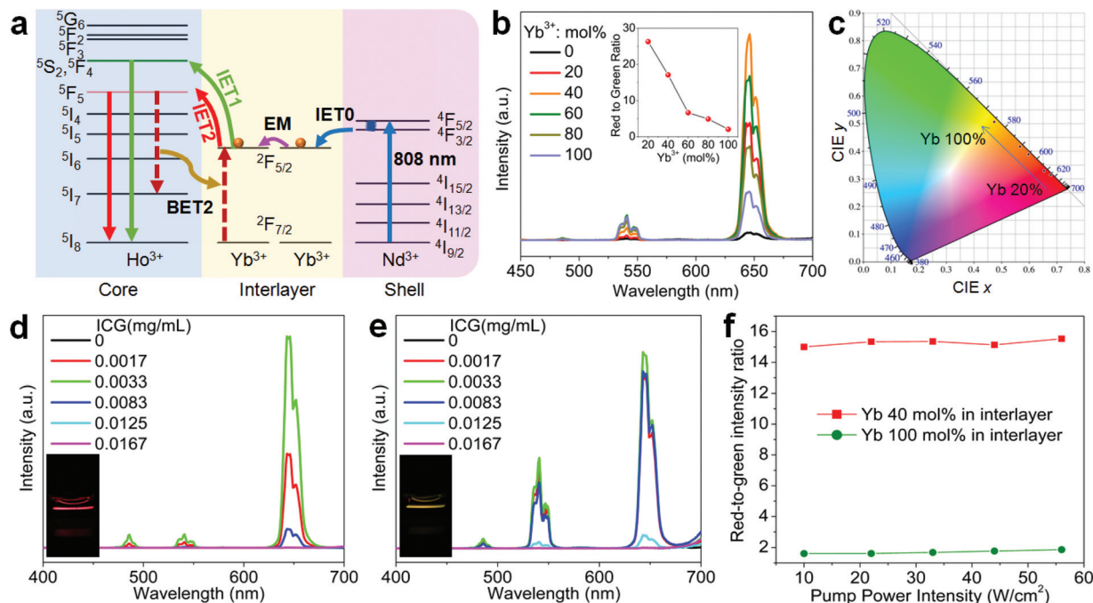
Fig. 6 (a) Schematic of using the nanostructure to manipulate the upconversion emission colors of the holmium lattice through core–interlayer interfacial energy transfer processes between Ho 3+ and Yb 3+ upon 808 nm excitation. (b) Upconversion emission spectra of as-prepared NaHoF 4 @NaYF 4 :Yb(0–100 mol%)@NaYF 4 :Nd/Yb(30/20 mol%) core–shell–shell nanoparticles under 808 nm excitation. Inset shows the dependence of the red-to-green emission intensity ratio as a function of the Yb 3+ concentration in the interlayer. (c) CIE coordinates of the emissions from (b) samples. (d and e) Upconversion emission spectra of (d) NaHoF 4 @NaYF 4 :Yb(40 mol%)@NaYF 4 :Nd/Yb(30/20 mol%) and (e) NaHoF 4 @NaYF 4 :Yb(30/20 mol%) with different ICG dye concentrations under 808 nm excitation. Insets show the corresponding emission photographs. (f) Dependence of upconversion red emission to green emission on pump power densities of 808 nm excitation for (d) and (e) samples.
