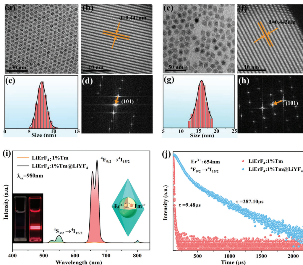
Fig. 1 TEM images, HRTEM images, particle size distribution, and the corresponding FFT of \text{LiErF}_4:1\%\text{Tm}^{3+} (a–d) and \text{LiErF}_4:1\%\text{Tm}^{3+}@ \text{LiYF}_4 (e–h) UCNP, respectively. (i) Upconversion emission spectra of \text{LiErF}_4:1\%\text{Tm}^{3+} and \text{LiErF}_4:1\%\text{Tm}^{3+}@ \text{LiYF}_4 UCNP under 980 nm excitation, the left inset shows the photographs of the corresponding samples under 980 nm excitation, and the right inset is the schematic illustration of the \text{LiErF}_4:1\%\text{Tm}^{3+}@ \text{LiYF}_4 core-shell structure. (j) The corresponding decay curves of \text{Er}^{3+} ions (654 nm) of \text{LiErF}_4:1\%\text{Tm}^{3+} and \text{LiErF}_4:1\%\text{Tm}^{3+}@ \text{LiYF}_4 UCNP under 980 nm excitation.
