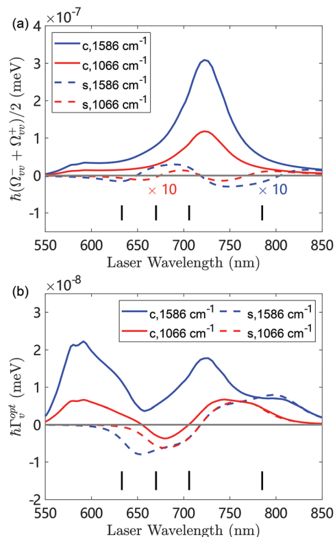
Fig. 5 (a) Vibrational frequency shift (\Omega_{\text{vw}}^+ + \Omega_{\text{vw}}^-)/2 and (b) effective optomechanical damping rate \Gamma_{\text{v}}^{\text{opt}} = \Gamma_{\text{vw}}^- - \Gamma_{\text{vw}}^+ as a function of the laser wavelength for the 1586\text{ cm}^{-1} vibrational mode (blue lines) and the 1066\text{ cm}^{-1} vibrational mode (red lines). The solid and dashed lines are the results from the continuum-field model (labeled as “c”) and the single-mode model (labeled as “s”), respectively. The vertical lines indicate wavelengths at 633 nm, 670 nm, 705.9 nm and 785 nm used for later simulations. The laser intensity is 1\text{ }\mu\text{W }\mu\text{m}^{-2} and other parameters are specified in the text.
