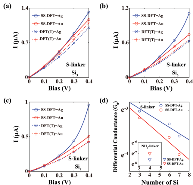
Fig. 3 I-V curves of the thiol-terminated silane junctions Si n -S-M calculated from the SS-DFT method. The I-V curves of Si n -S-M calculated from the SS-DFT method are shown in (a) for n = 3 (Si 3 ), (b) for n = 6 (Si 6 ) and (c) for n = 7 (Si 7 ). SS-DFT-Au/Ag denotes SS-DFT results for Si n -S-Au/Ag. As a reference, I-V curves from TransSIESTA (DFT(T)) are also shown (dotted lines in the figures). Note that at small biases ( \leq 0.1 V), there are no essential differences between the two methods. Significant differences occur at biases > 0.1 V. (d) Differential conductance of Si n -S-M (M = Au or Ag) at 0.2 V calculated from SS-DFT for n = 3, 6 and 7. The two solid lines in the figure are obtained by linear fitting. Inset: differential conductance of Si n -NH 2 -M (M = Au or Ag) at 0.2 V from SS-DFT. For the NH 2 linker, the Au contact is more conducting than the Ag contact. The trend reverses for the S linker.
