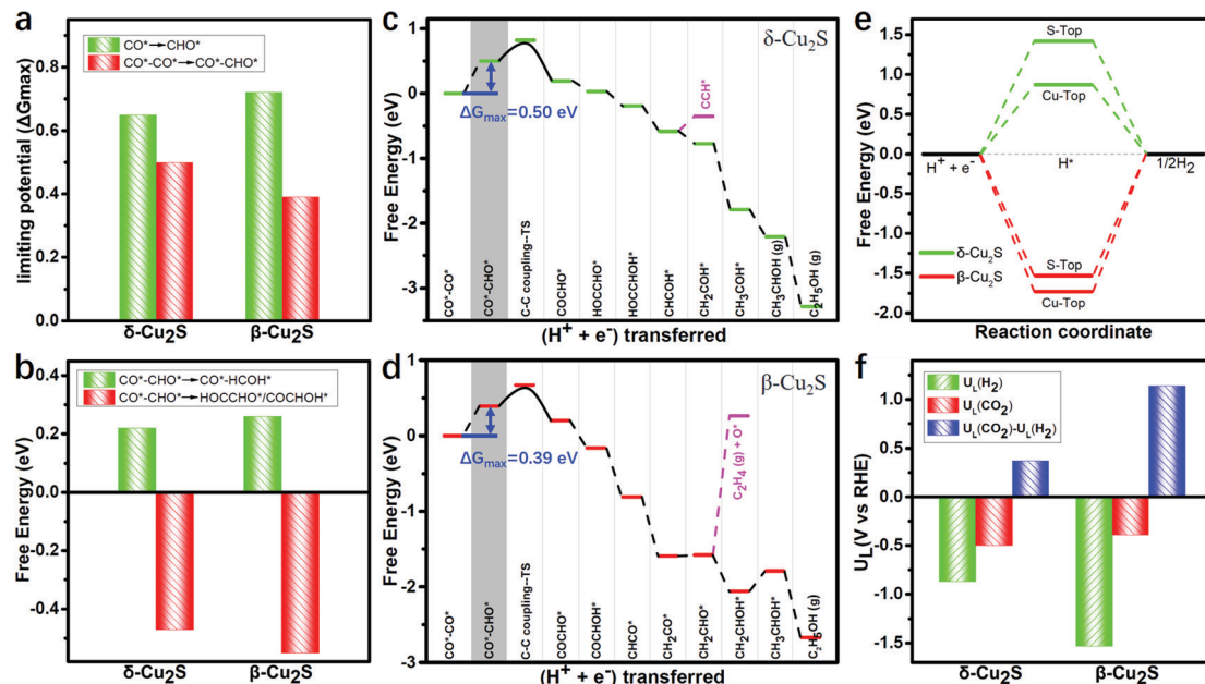
Fig. 3 Free energy of the hydrogenation step of (a) CO* \rightarrow CHO* and CO* \rightarrow CHO* \rightarrow HOCCHO*/COCHOH*. Free energy diagrams of CO* \rightarrow CHO* hydrogenation to C 2 H 5 OH on (c) \delta -Cu 2 S and (d) \beta -Cu 2 S. Limiting potential is obtained from the maximum free energy change ( \Delta G_{\text{max}} ) of the whole reaction process, which is marked by blue lines. (e) Free energy profiles of the HER on \delta -Cu 2 S (green line) and \beta -Cu 2 S (red line). (f) Limiting potentials for the CO 2 RR U_L(\text{CO}_2) , HER U_L(\text{H}_2) and difference U_L(\text{CO}_2) - U_L(\text{H}_2) on \delta -Cu 2 S and \beta -Cu 2 S monolayers.
