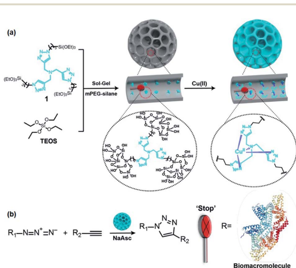
Fig. 45 (a) Cu-TTASi nanoreactors and the detailed coordination relations of Cu II and \text{N}(\text{C}_3\text{N}_3)_3 ligands and (b) Cu I -TTASi-catalyzed CuAAC reactions in the presence of sodium ascorbate. mPEG-silane: PEGylation triethoxysilane; NaAsc: sodium ascorbate. 235 Reproduced with permission. 235 Copyright 2021, American Chemical Society.
