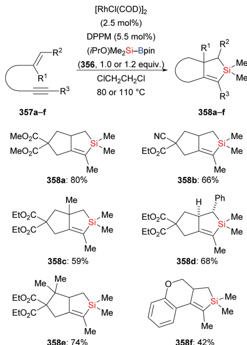
Scheme 117 Rhodium-catalysed (2+2+1) cycloaddition.
