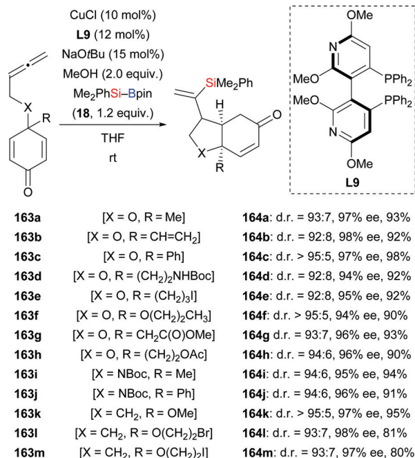
Scheme 46 Copper-catalysed enantioselective silylative cyclization of allenones to access bicyclo[4.3.0]nonanes.
