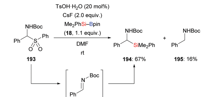
Scheme 61 Metal-free synthesis of α-aminosilanes from imine precursors.
