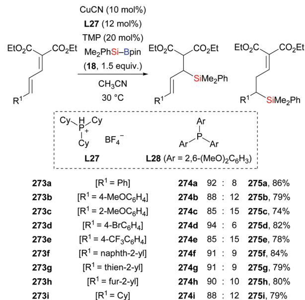
Scheme 83 Copper-catalysed silylation of electron-deficient alkynes. Yields are for the mixture of isomers.
