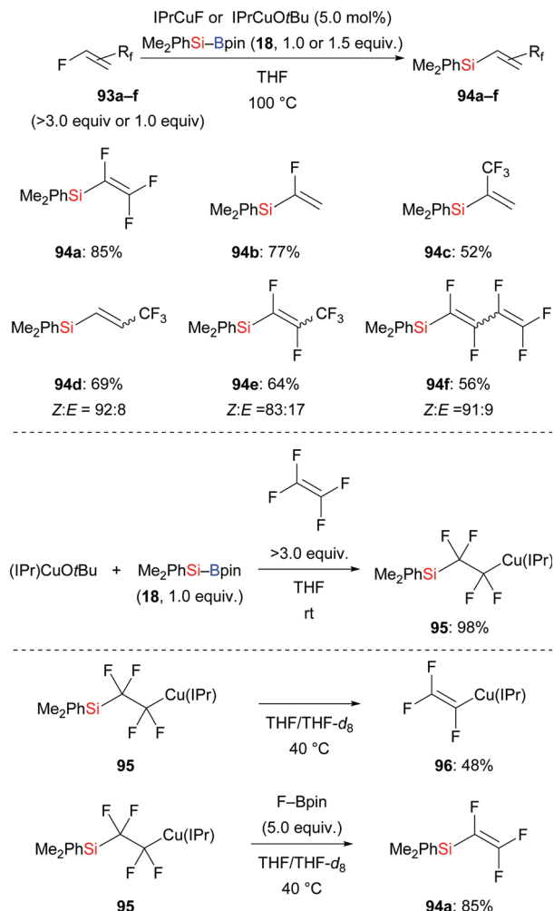
Scheme 29 Copper-catalysed defluorosilylation of fluoroalkenes.
