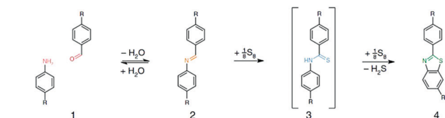
Fig. 1 General scheme of the topochemical conversion of the imine bond into the thiazole-linkage in TTT-COF. Reproduced with permission. 37 Copyright 2018, Nature Publishing Group.
