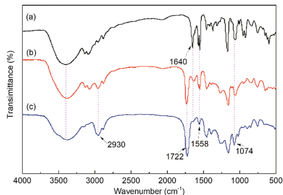
Fig. 1 The FT-IR spectra of (a) VHPIImBr, (b) s -PIL-2 and (c) HPIL-7.
