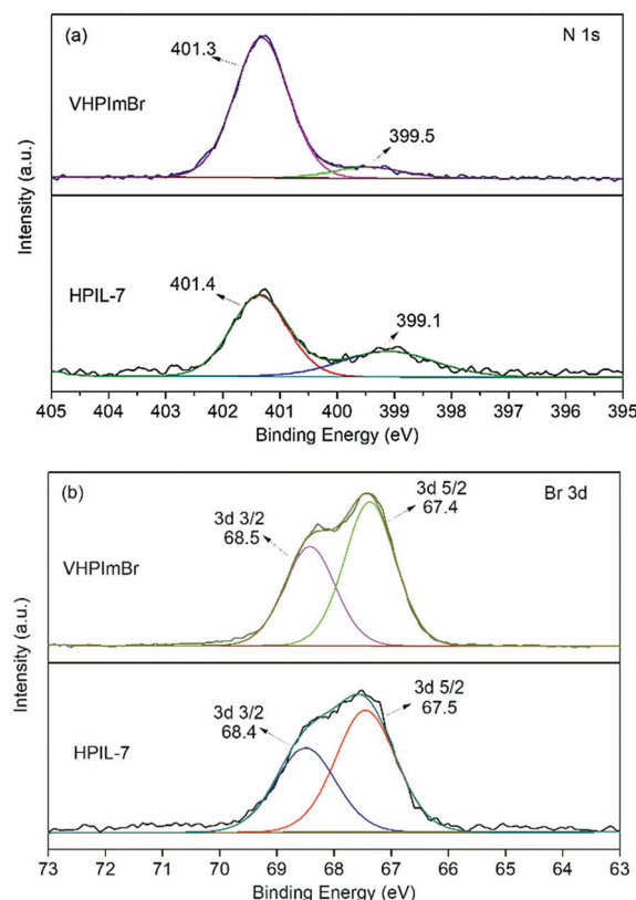
Fig. 2 XPS spectra of N 1s and Br 3d for VHPIImBr and HPIL-7.
