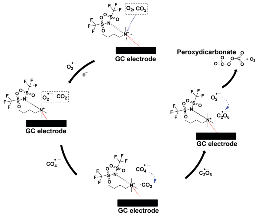
Scheme 2 The proposed mechanism of \text{CO}_2 utilization by \text{O}_2^{\bullet-} in [BMAm + ][TFSI - ].
