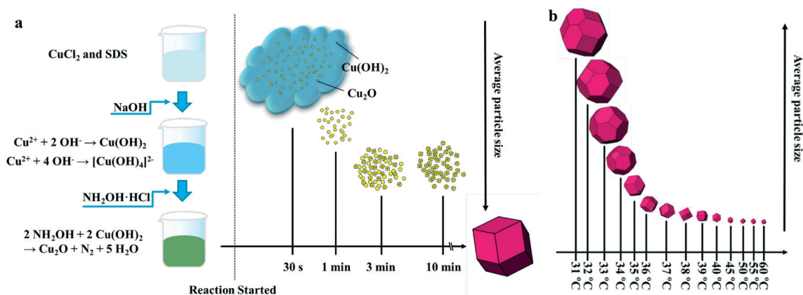
Fig. 1 (a) Schematic diagram of particle size and morphology evolution of d- \text{Cu}_2\text{O} with increasing reaction time synthesized at a specific temperature. (b) Schematic diagram of particle size and morphology evolution of d- \text{Cu}_2\text{O} with increasing synthesis temperature.
