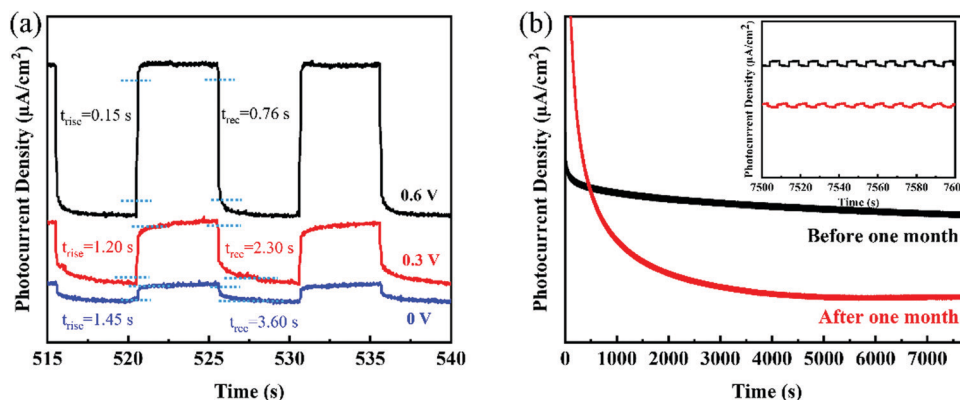
Fig. 4 (a) The photocurrent density versus time for the rise ( t_{\text{ris}} ) and recovery ( t_{\text{rec}} ) times of the 2D GeNS-based photodetector with three applied voltages (0, 0.3 and 0.6 V). (b) Stability of photo-response behaviours of the 2D GeNS-based photodetector with 8000 s and one-month duration with 0.5 M KOH and at voltages of 0.6 V. (b) Enlarged 100 s cycles from 7500–7600 s.
