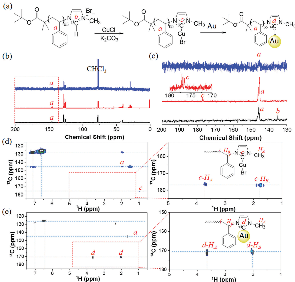
Fig. 3 (a) Synthesis of ^{13}\text{C} -labeled \text{PS}_{65}\text{-}^{13}\text{C-NHC-Au} using ^{13}\text{C} -Im. (b and c) ^{13}\text{C} NMR spectra of \text{PS}_{65}\text{-}^{13}\text{C-NHC-Cu(i)} (red, middle) and \text{PS}_{65}\text{-}^{13}\text{C-NHC-Au} (blue, top) in \text{CDCl}_3 . ^{13}\text{C} NMR spectra in (b) in the range of 130–200 ppm is zoomed in (c). (d) 2D HMBC spectrum of non-labeled \text{PS}_{65}\text{-NHC-Cu(i)} . (e) 2D HMBC spectrum of ^{13}\text{C} -labeled \text{PS}_{65}\text{-}^{13}\text{C-NHC-Au} .
