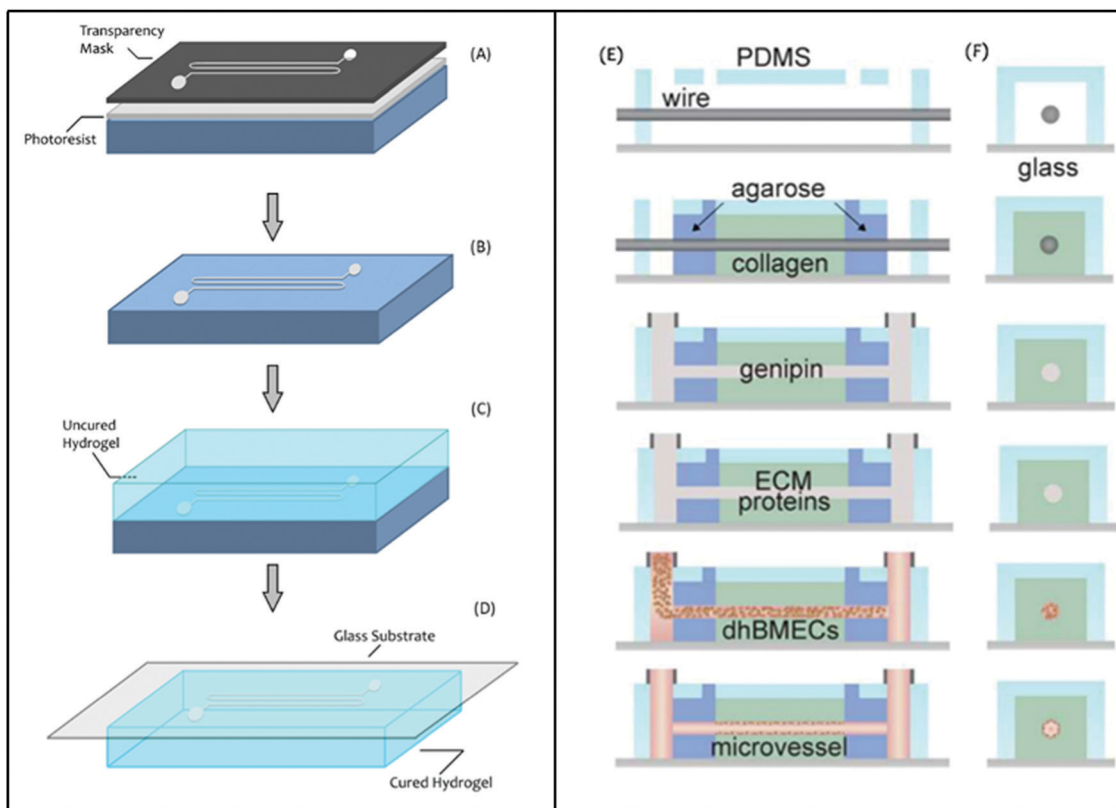
Fig. 4 Using molds to make microfluidic channels in hydrogels. (A) Applying a mask on top of a photoresist (SU-8) layer so that only the exposed region is crosslinked. (B) Removing the uncured photoresist to have raised microstructures. (C) A hydrogel is cast on top of the mold, cross-linked, and an imprint of the microstructure is left in the casting material. (D) A substrate, often glass, is pressed onto the cast hydrogel to seal the channel. (E and F) Fabrication of microchannels using a wire mold (150 \mu\text{m} diameter). Collagen and agarose were gelled around the suspended wire; when the wire was removed a channel is left in the hydrogel which was seeded with differentiated human brain microvascular endothelial cells (dhBMECs). Reprinted with permission from Linville et al. (2019).
