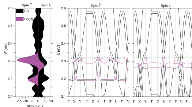
Fig. 5 DFT calculations. Electronic band structure based on the crystal structure determined by using DFT calculations. High symmetry points in the crystal reciprocal lattice: T = (0, 0, 0) , X = (0.5, 0, 0) , Y = (0, 0.5, 0) , Z = (0, 0, 0.5) , R = (0.5, -0.5, 0.5) , T = (0, 0.5, -0.5) , U = (0.5, 0, -0.5) , and V = (0.5, -0.5, 0) . The Fermi energy level (green dashed line) is set at 2.32 eV. The magenta and black areas and curves indicate Co and BO electrons, respectively.
