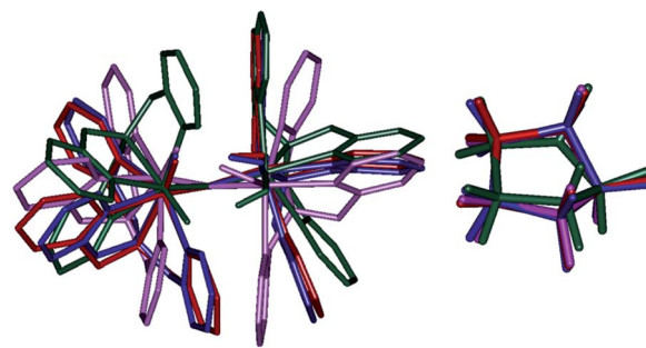
Fig. 10 Structural overlay of ^2\text{RC}_{\text{hs-hs}} (blue), \text{I-}^2\text{TS}_{\text{Hhs-hs}} (red), \text{II-}^2\text{TS}_{\text{Hhs-hs}} (dark green), and \text{III-}^2\text{TS}_{\text{Hhs-hs}} (magenta) and their corresponding cyclopentane ring (right) shown separately. H atoms are omitted for clarity.
