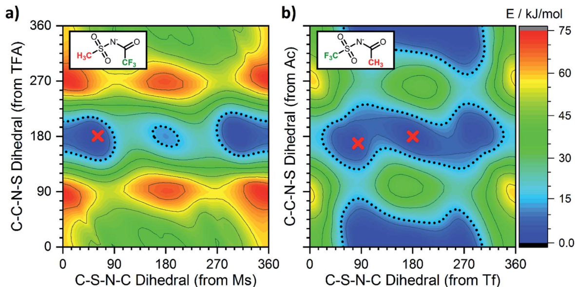
Fig. 13 Potential energy surfaces of the anions (a) [\text{N}(\text{Ms})(\text{TFA})]^- and (b) [\text{N}(\text{Tf})(\text{Ac})]^- in the experimentally investigated ILs. The red crosses correspond to the dihedral angles obtained experimentally from crystal structures of model compounds.
