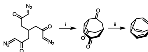
Scheme 2 Serratos's stepwise BV synthesis. 12 Reagents and conditions: (i) CuSO 4 , PhSMe, xylene, 140 °C, \sim 2\% ; (ii) (1) TsNHNH 2 , (2) MeLi, 20%.
