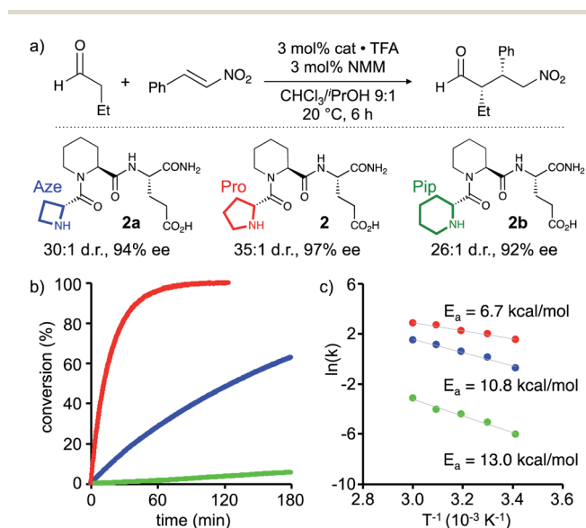
Scheme 2 (a) Conjugate addition reaction of butanal to nitrostyrene catalyzed by 2a , 2 and 2b . (b) In situ IR monitoring of the formation of γ-nitroaldehyde, and (c) Arrhenius plot and activation energy of the peptide catalyzed reactions.
